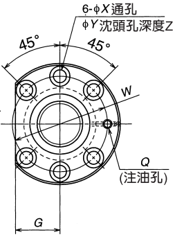
俯視X-X
