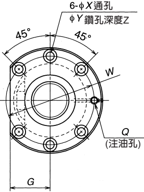
俯視X-X
