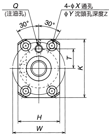
俯視X-X
